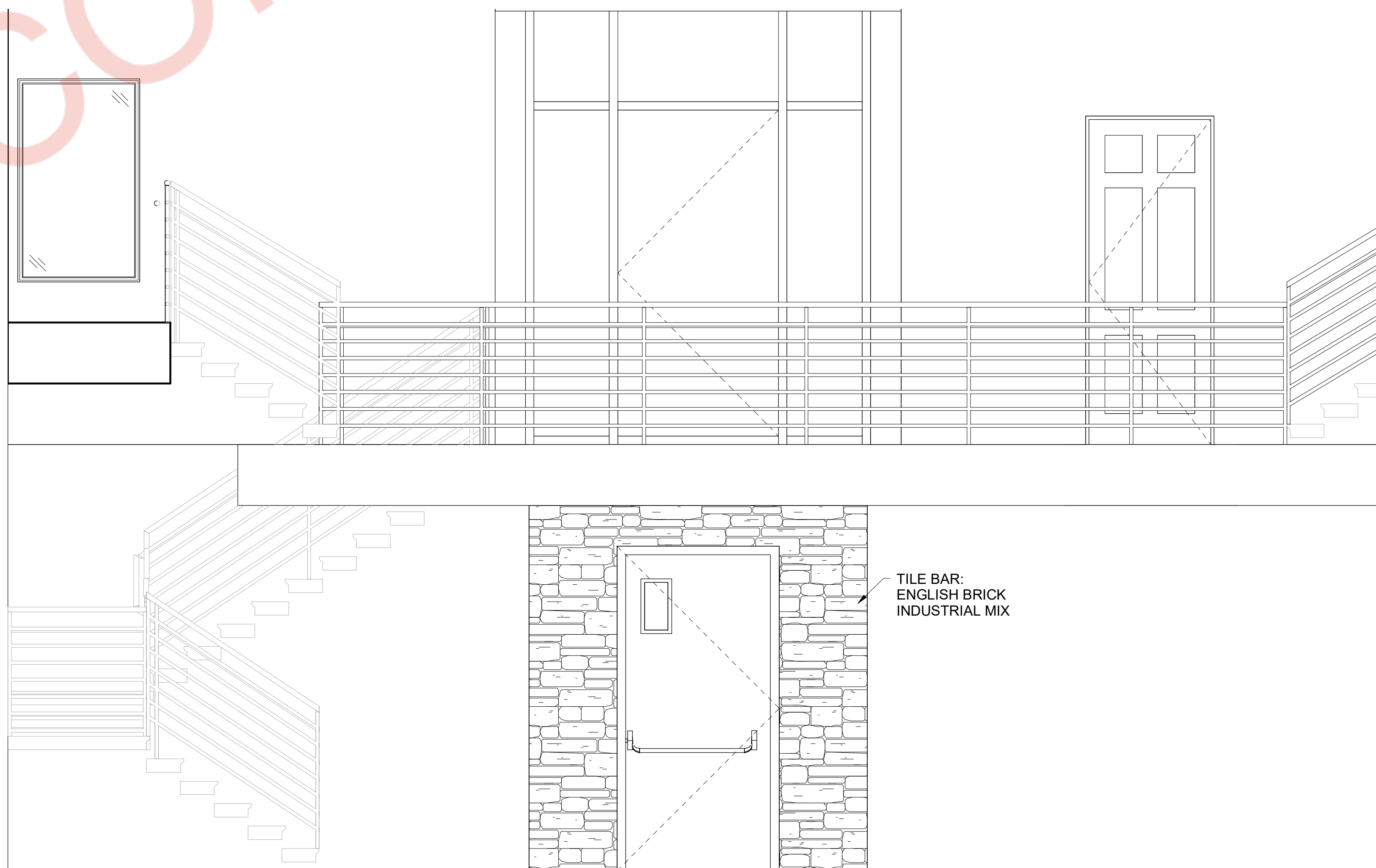
3 STAIR WALL ELEVATION ID103 1/2" = 1'-0"
