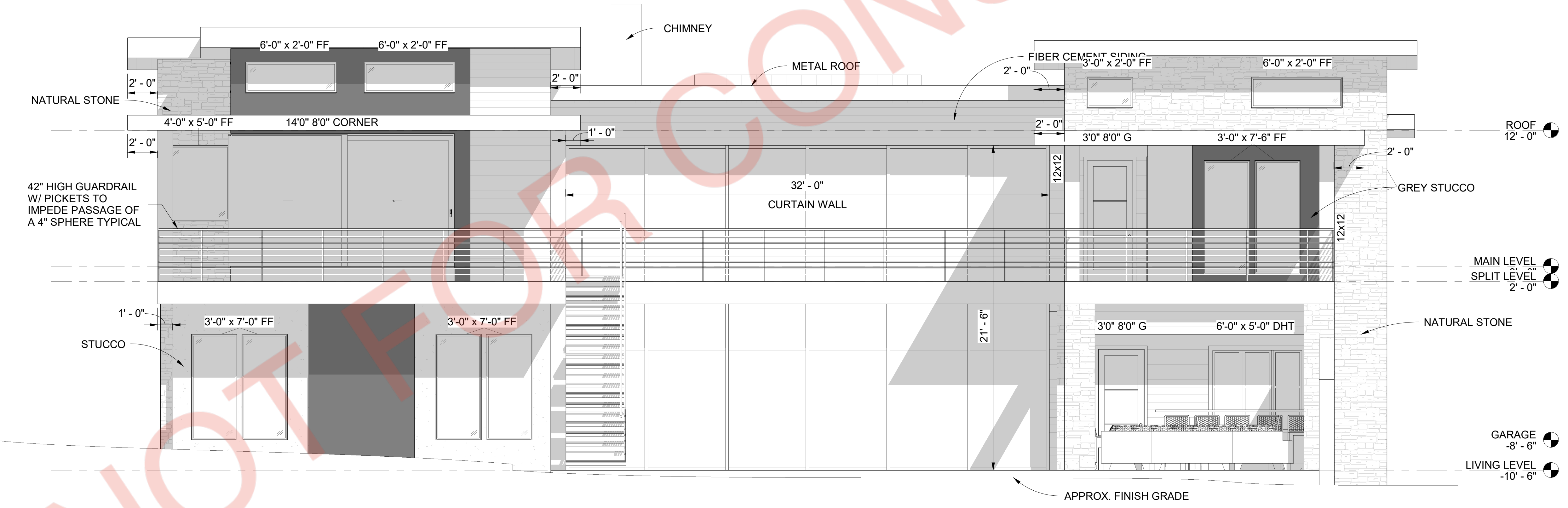
2 REAR ELEVATION 1/4" = 1'-0"
