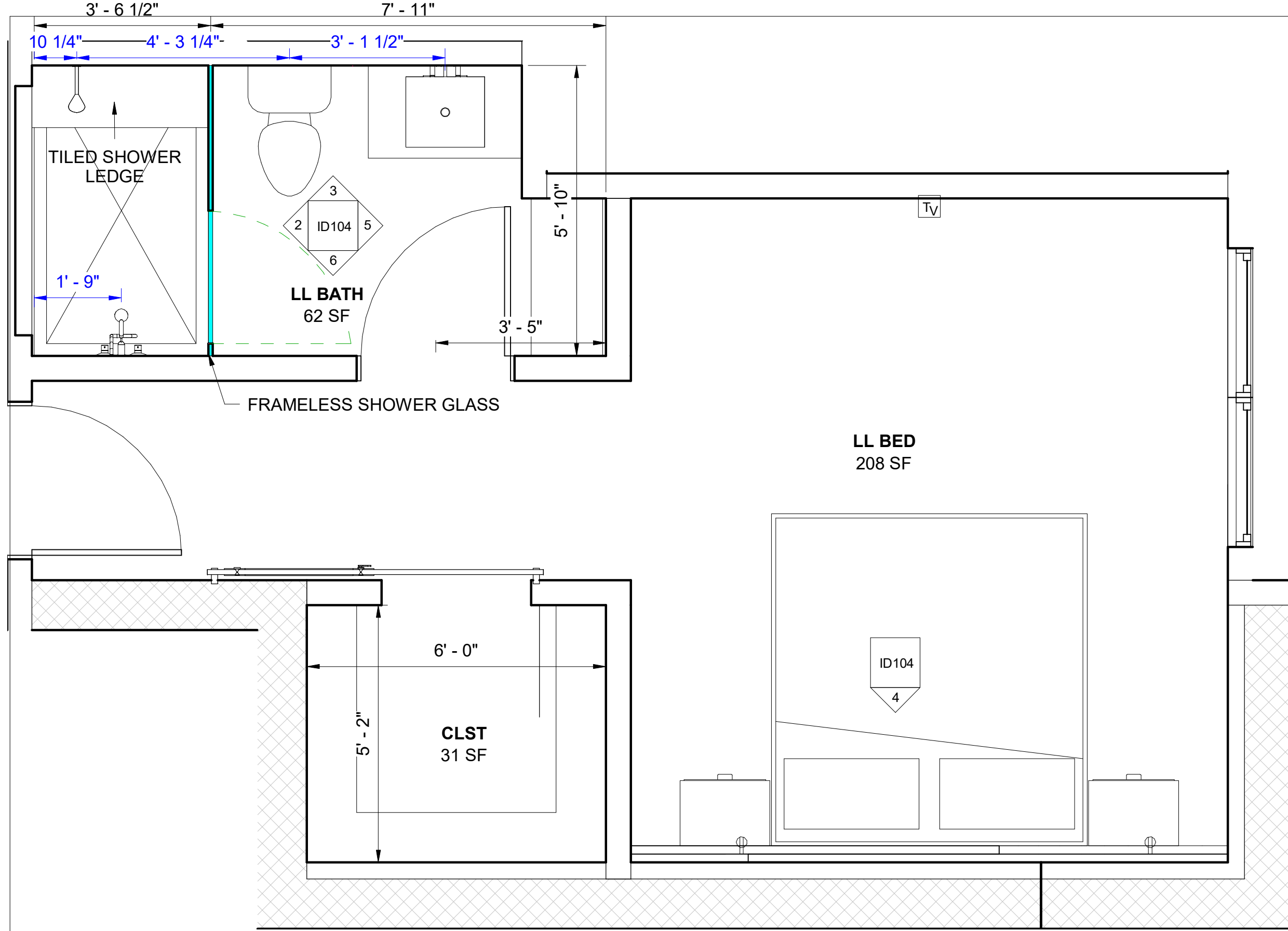
1 LIVING LEVEL - EXTRA BED/BATH ID104 1/2" = 1'-0"
