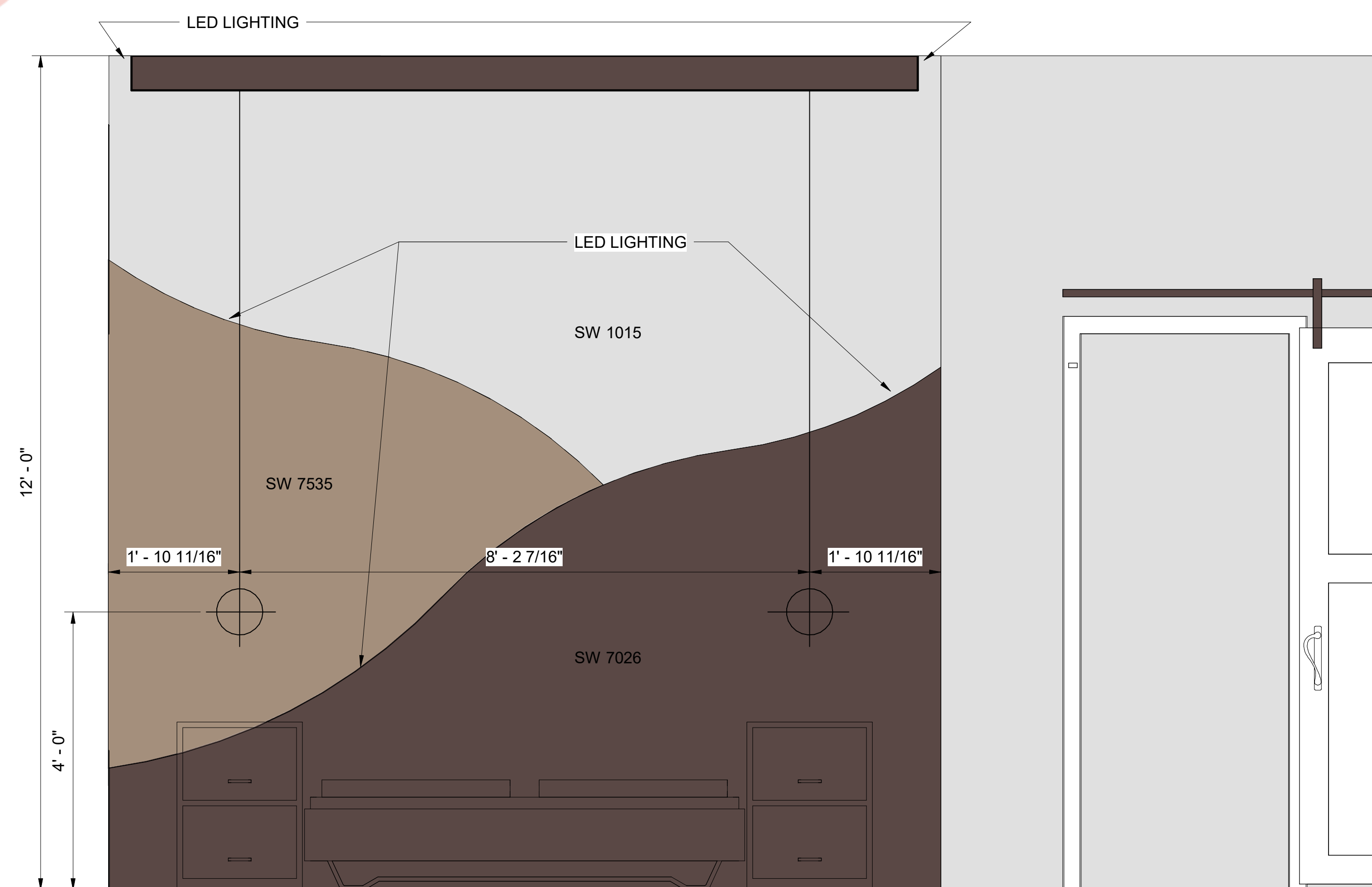
4 EXTRA BED ELEVATION ID104 3/4" = 1'-0"
