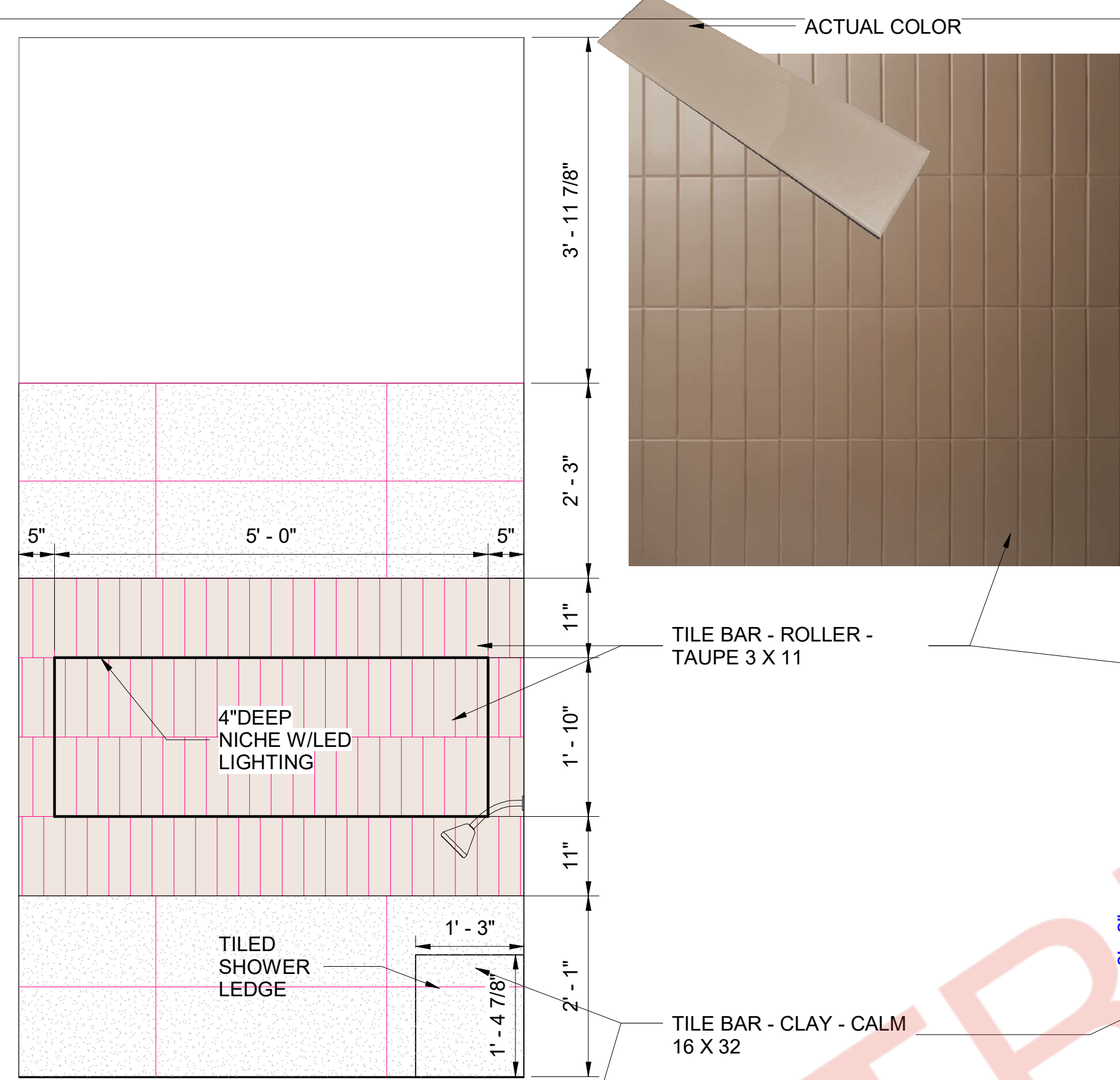
2 EXTRA BATH SHOWER NICHE ID104 3/4" = 1'-0"
