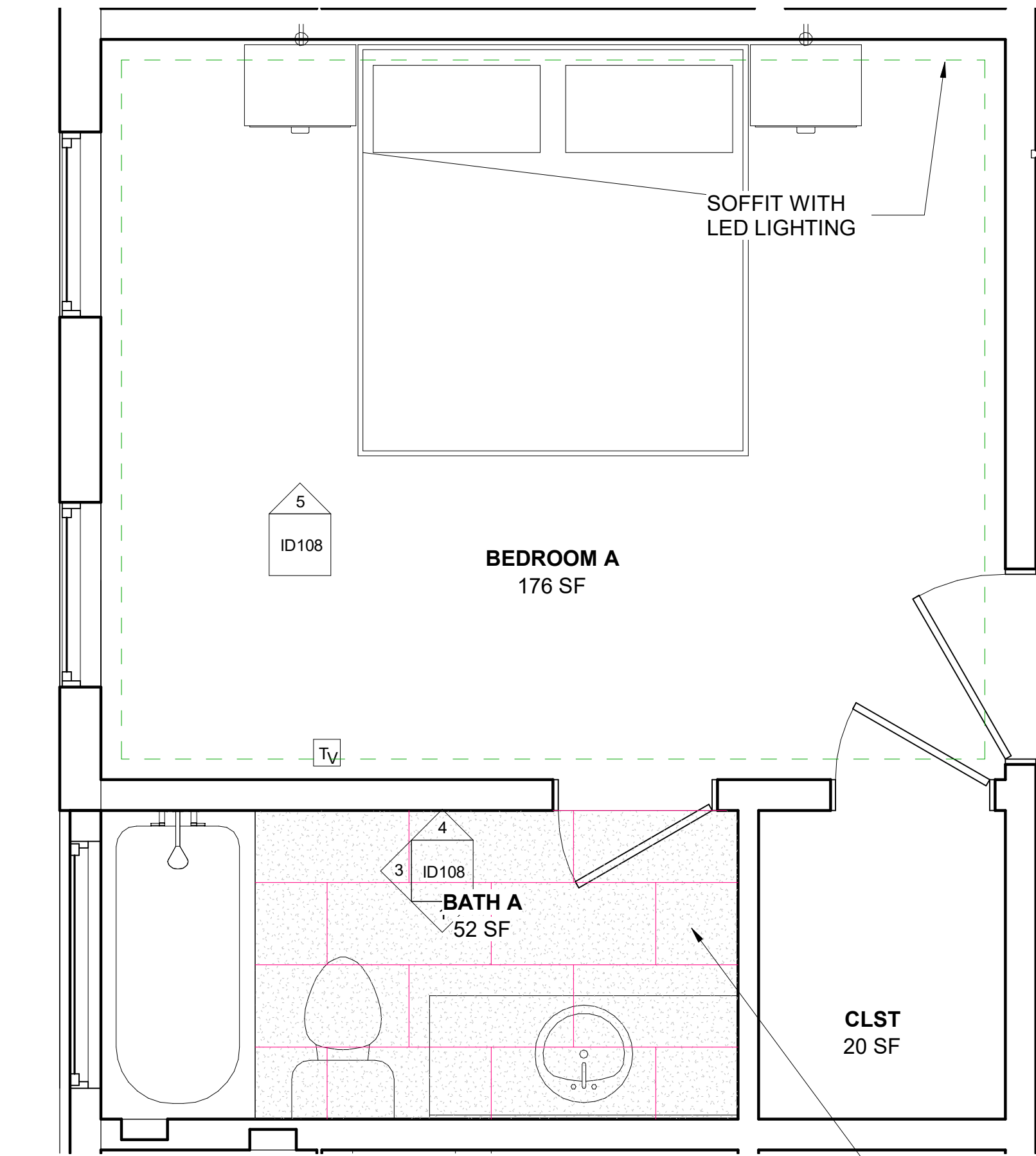
2 MAIN LEVEL - BEDROOM A 1/2" = 1'-0"
