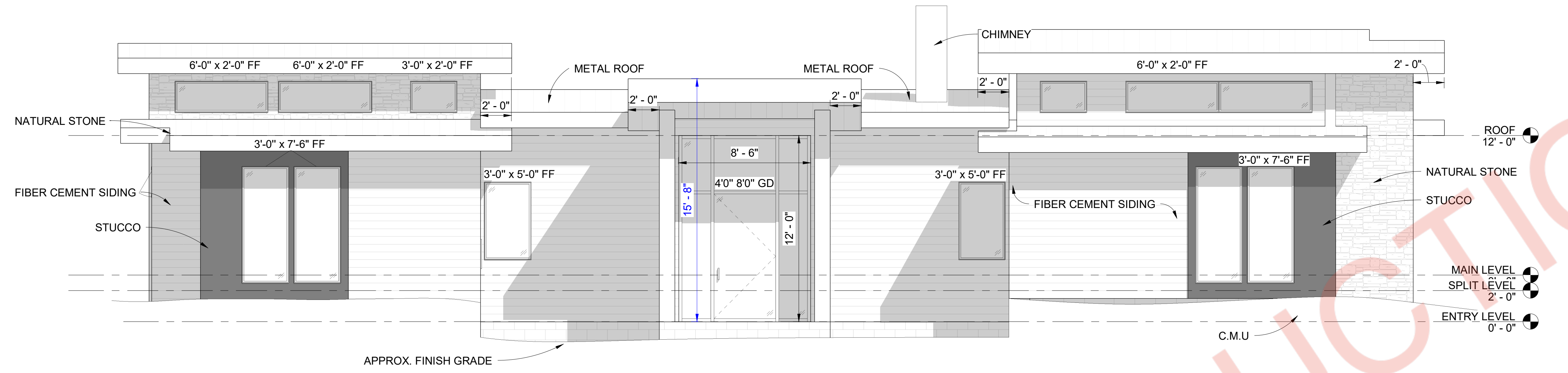
1 FRONT ELEVATION 1/4" = 1'-0"
