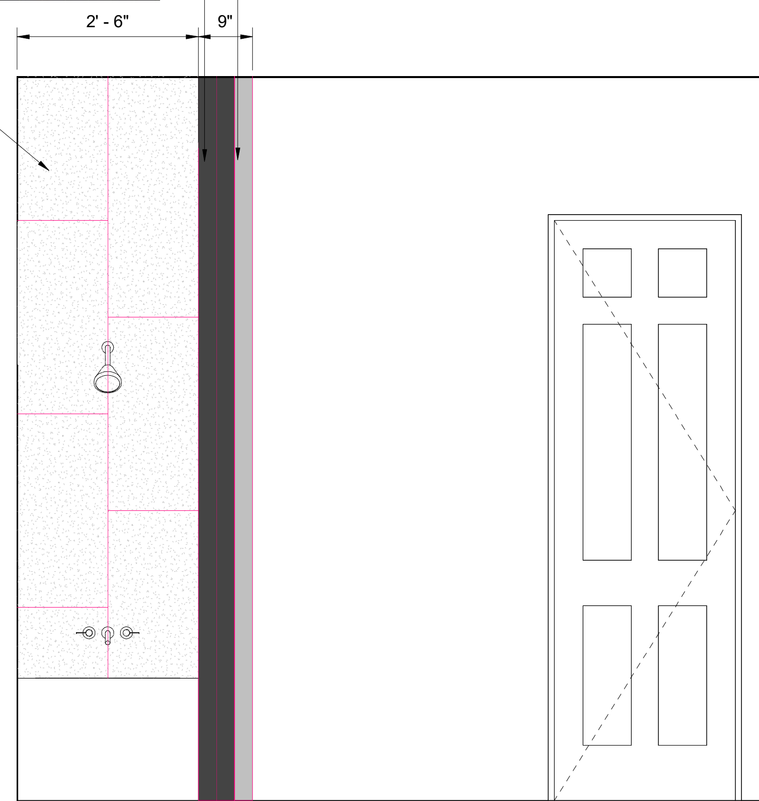
4 BATH A - SHOWER WALL 3/4" = 1'-0"
